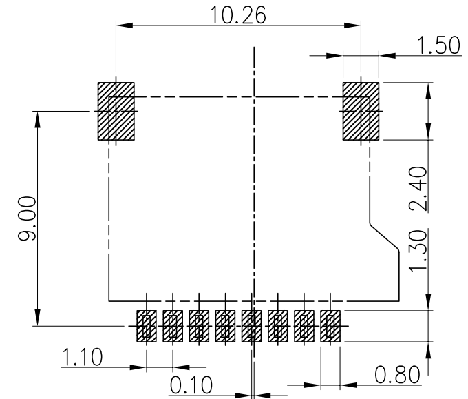
RECOMMENDED PCB LAYOUT (Witchout Post)
